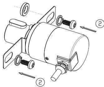
Absolute Encoder
